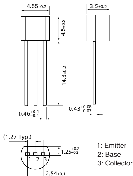
TO-92
